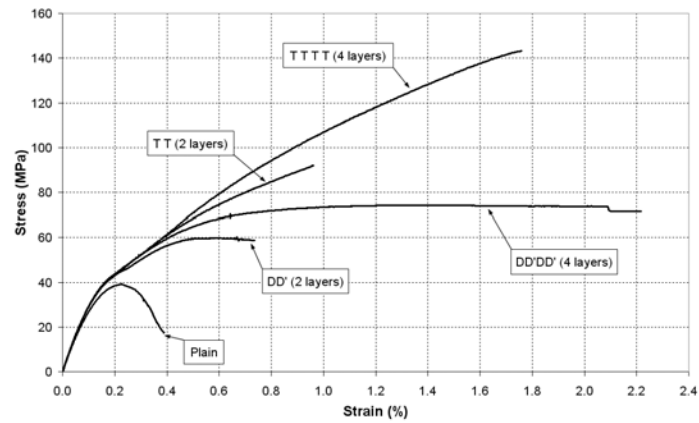
Figure 8 Behavior of wrapped specimens with angle orientation
