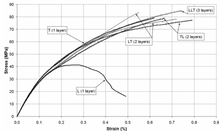
Figure 7 Combination of transverse and longitudinal orientations
