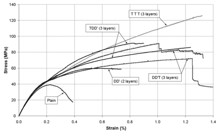
Figure 9 Combination of angle and transverse orientation
