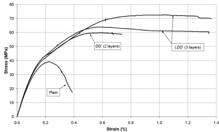
Figure 10 Combination of angle and longitudinal orientation
