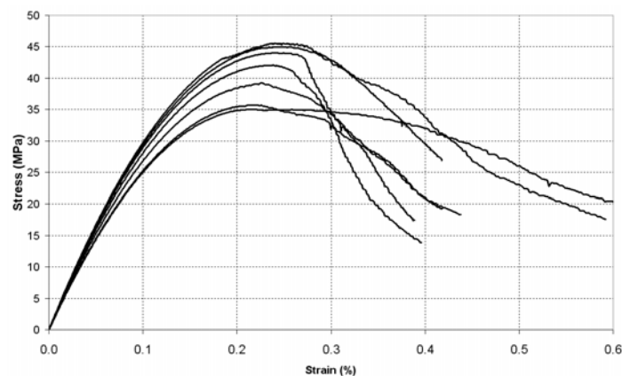
Figure 3 Stress-strain behavior of plain specimens
