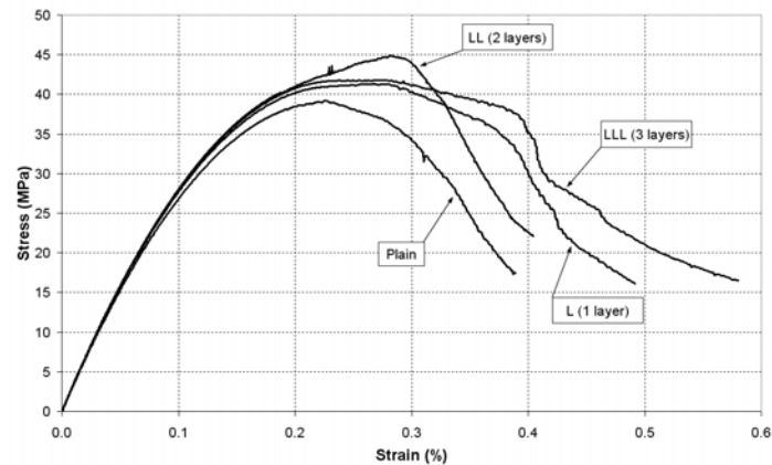
Figure 6 Behavior of specimens with longitudinal orientations
