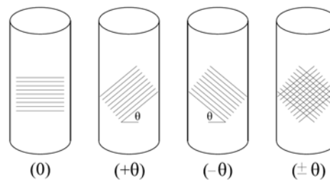
Figure 1 Fiber orientation in CFRP-wrapped cylinders [5]
