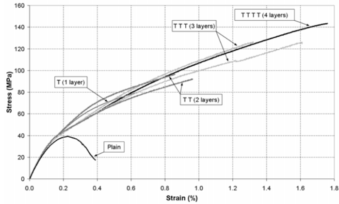
Figure 5 Behavior of wrapped specimens with hoop orientations
