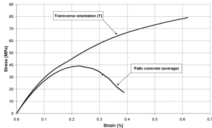
Figure 4 Behavior of one layer wrapped specimen in hoop direction
