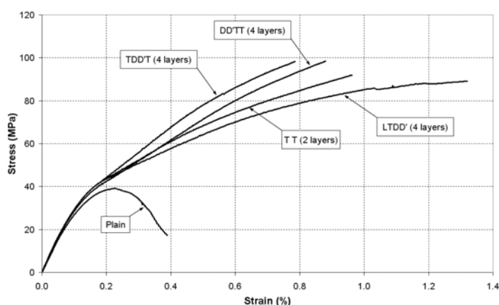
Figure 11 Specimens with combination orientation
