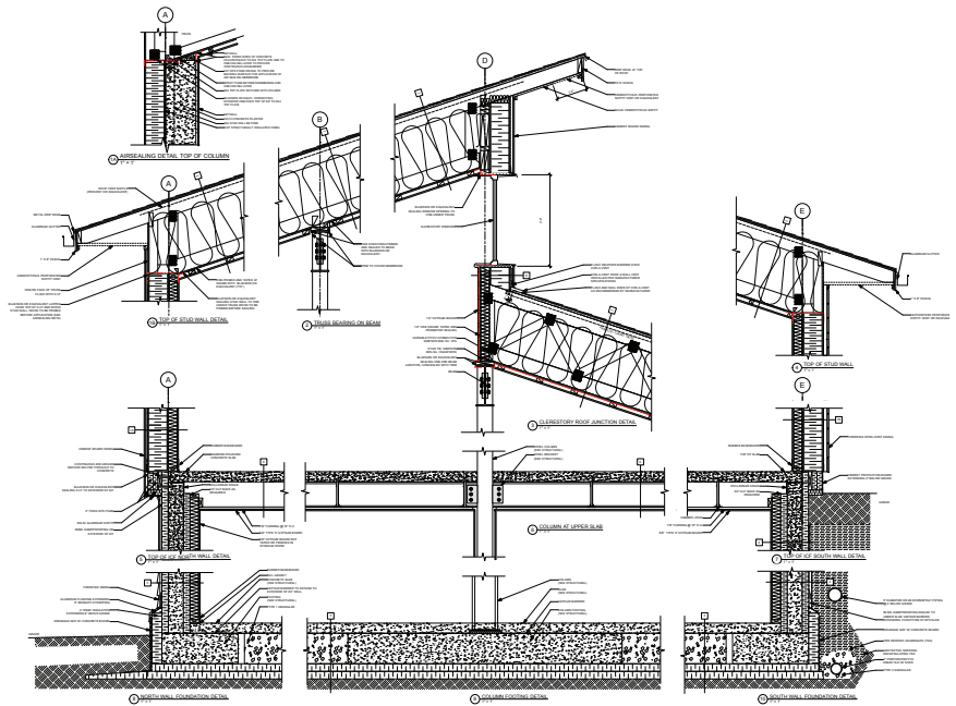
Construction Details, VWRM Passive House Office, Solterre Design.
